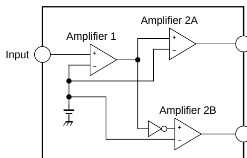
Figure 1 Amplifier Configuration
