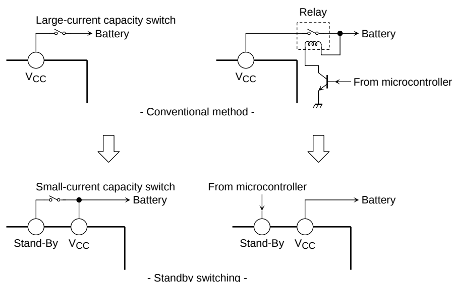
Figure 3 Standby switching
