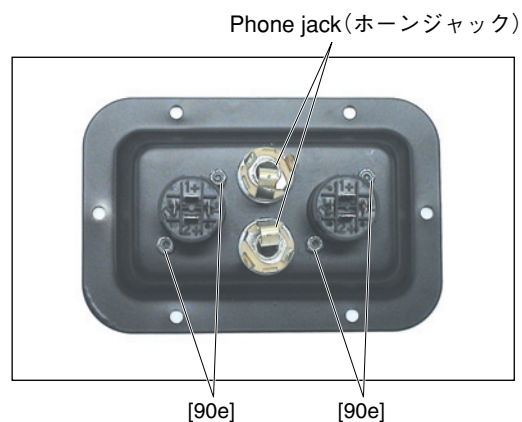
[90e]: Hexagonal Nut (六角ナット) #4-40 NYLOK NUT (WJ372000)
