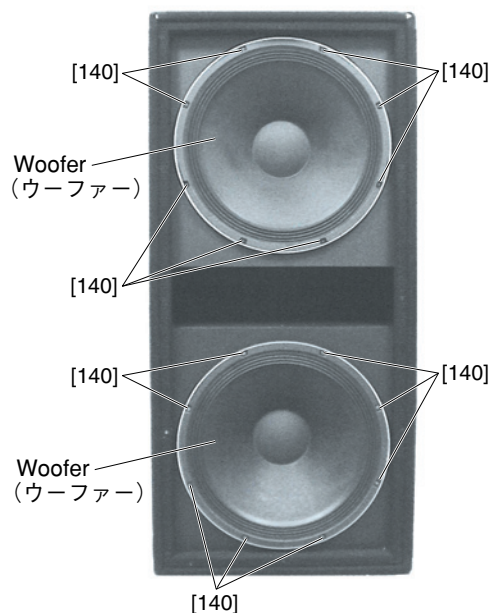
[140]: PAN HD Machine Screw (鍋ねじ) #10-32 x 1-1/2 (WJ624200)
