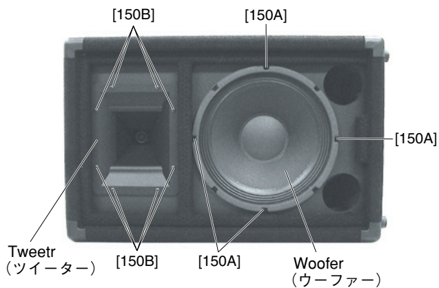
[150]: Pan Head PB Screw (鍋ねじ) PHPBS #8 x 1 BLK (WJ911500)
