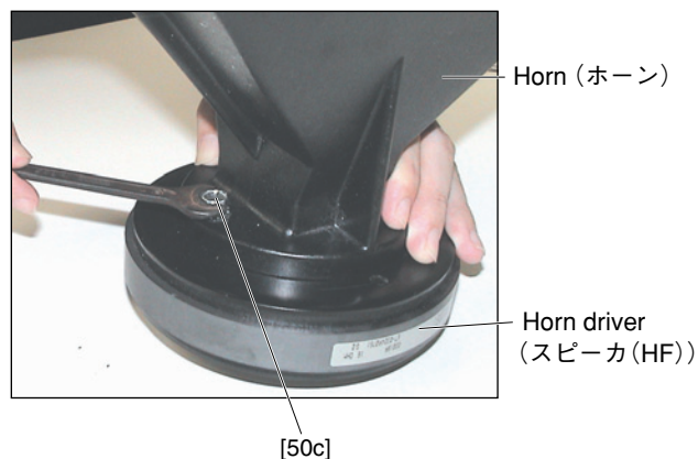
[50c]: Hex Head Mach Screw (歯付座金付六角ボルト) 1/4 x 5/8 inch (WJ356300)
