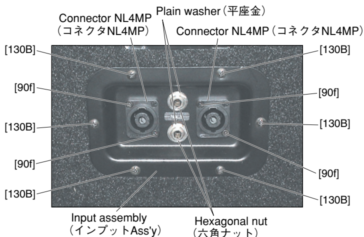
[90f]: FH Machining Screw (皿ねじ) #4-40 x 3/8 ZN BL (WJ372100)
