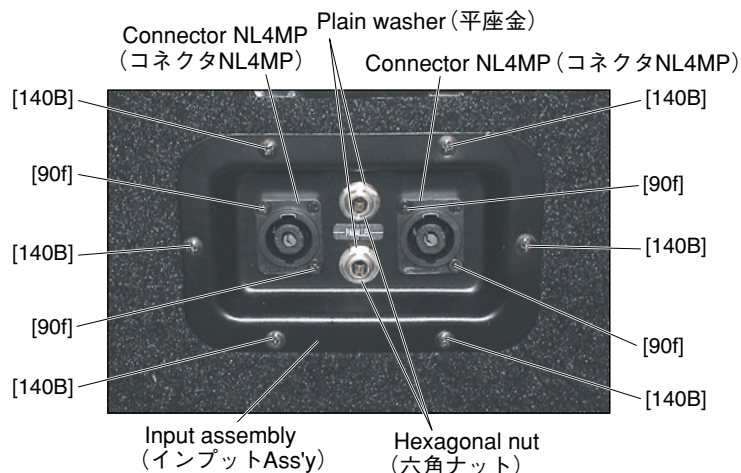
[90f]: FH Machining Screw (皿ねじ) #4-40 x 3/8 ZN BL (WJ372100) [140]: TH Sheet Metal Screw (トラスタップねじ) #6 x 5/8 BLK (WJ493800)
