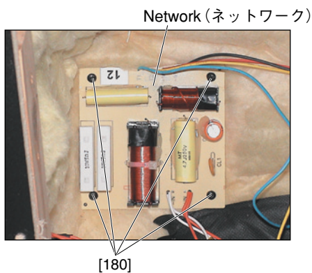
[180]: Pan Head SM Screw (鍋ねじ) PHSMS #6 x 3/4 BLK (WJ911700)
