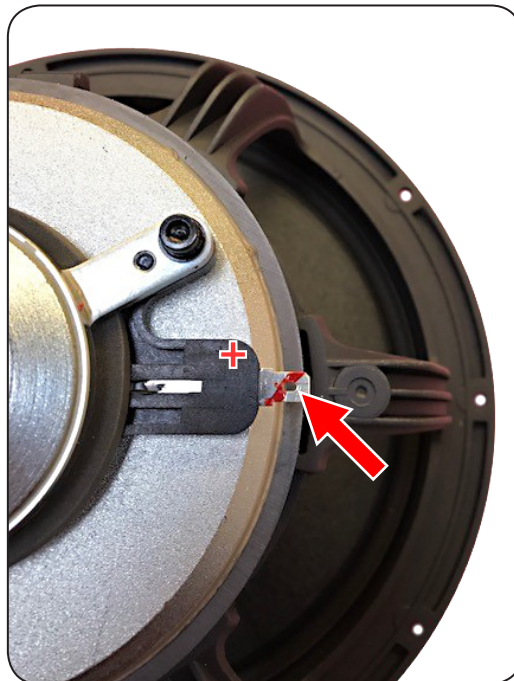
Green wire (Negative) to be connected to the positive terminal
