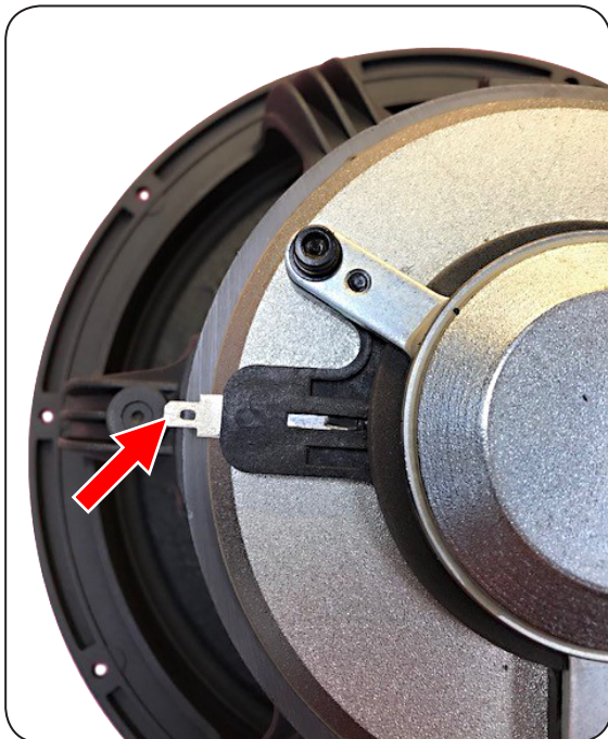
Yellow wire (Positive) to be connected to negative terminal
