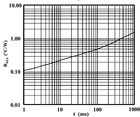
R_{\theta JA} vs. t
