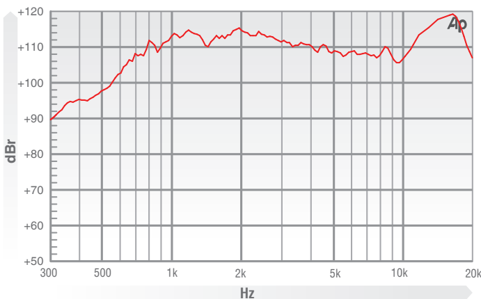
Frequency response measurement taken on axis with 1w signal at distance of 1M using custom horn with 80° x 60° coverage
